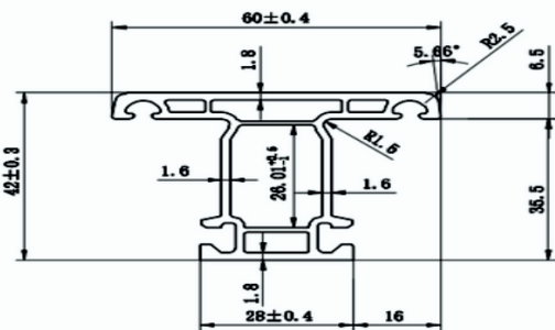
SLIDING T-MULLION
