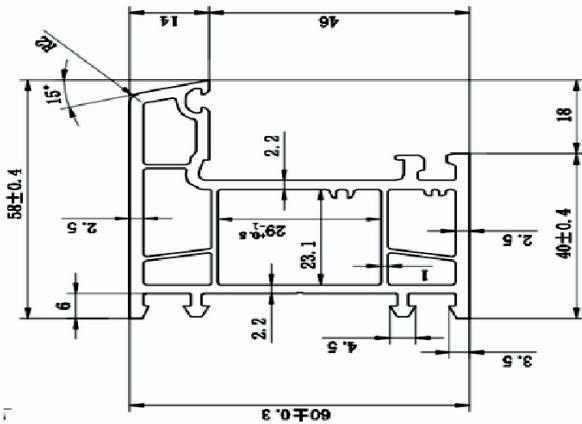
CASEMENT OUTER FRAME
