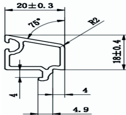
CASEMENT DOUBLE GLASS BEADING
