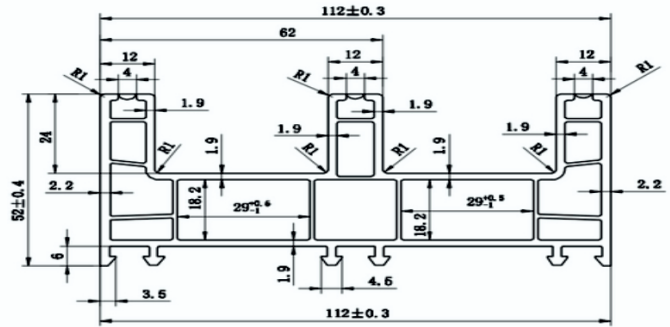
3 TRACK SLIDING FRAME
