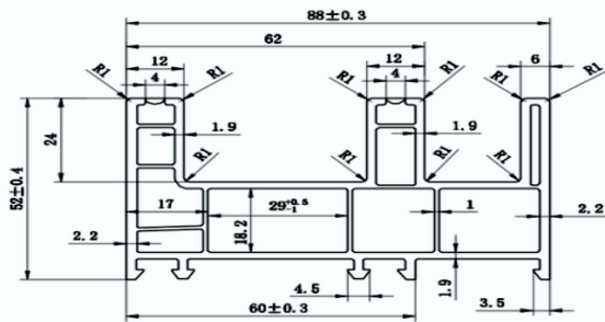
2.5 TRACK FRAME
