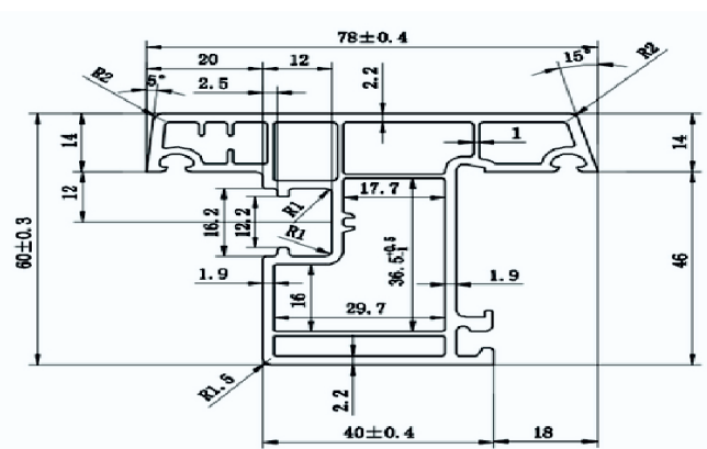
CASEMENT WINDOWS SASH OUTWARD
