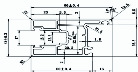
SLIDING WINDOWS SASH
