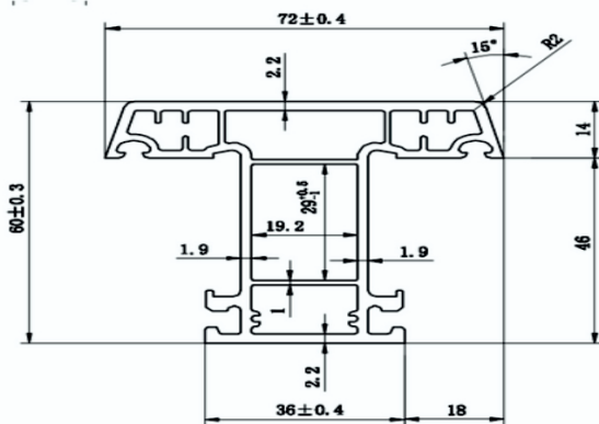
CASEMENT DOOR SASH OUTWARD
