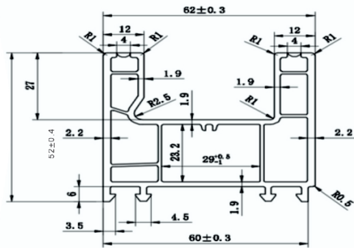
2 TRACK SLIDING FRAME
