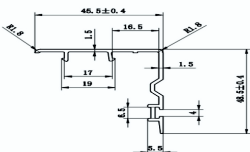
SLIDING SINGLE GLAZING BEAD
