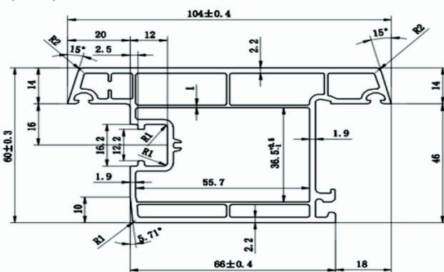
CASEMENT DOOR SASH OUTWARD
